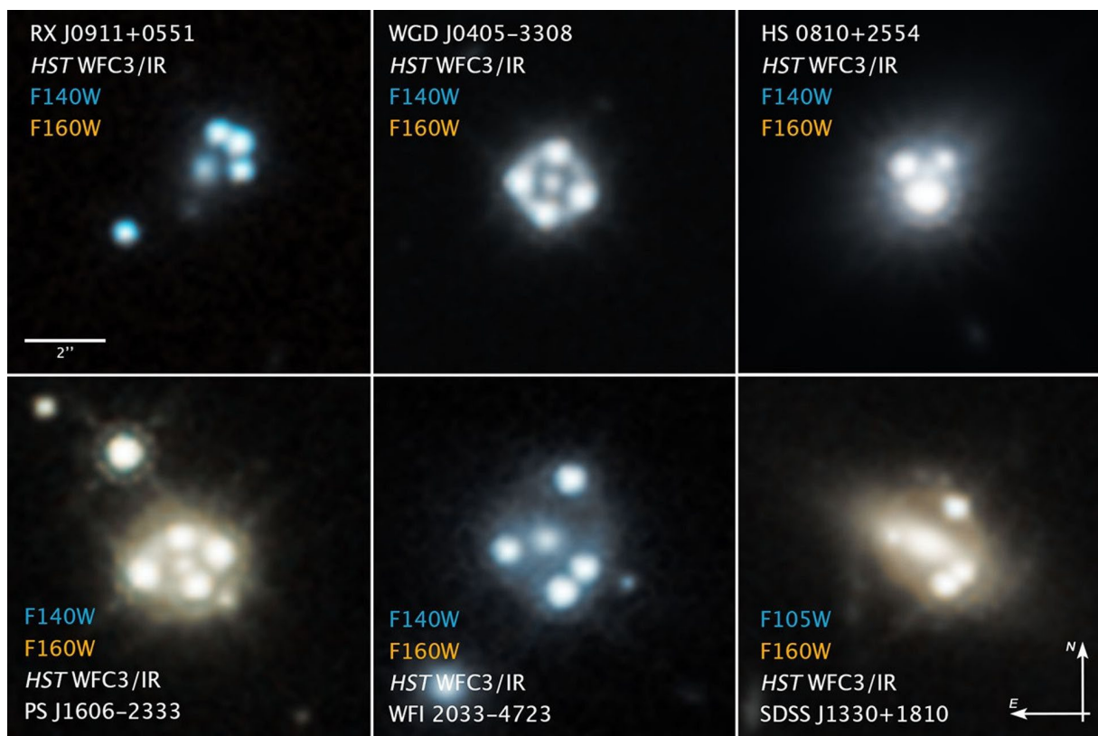
Compass Image of Gravitationally Lensed Quasars
