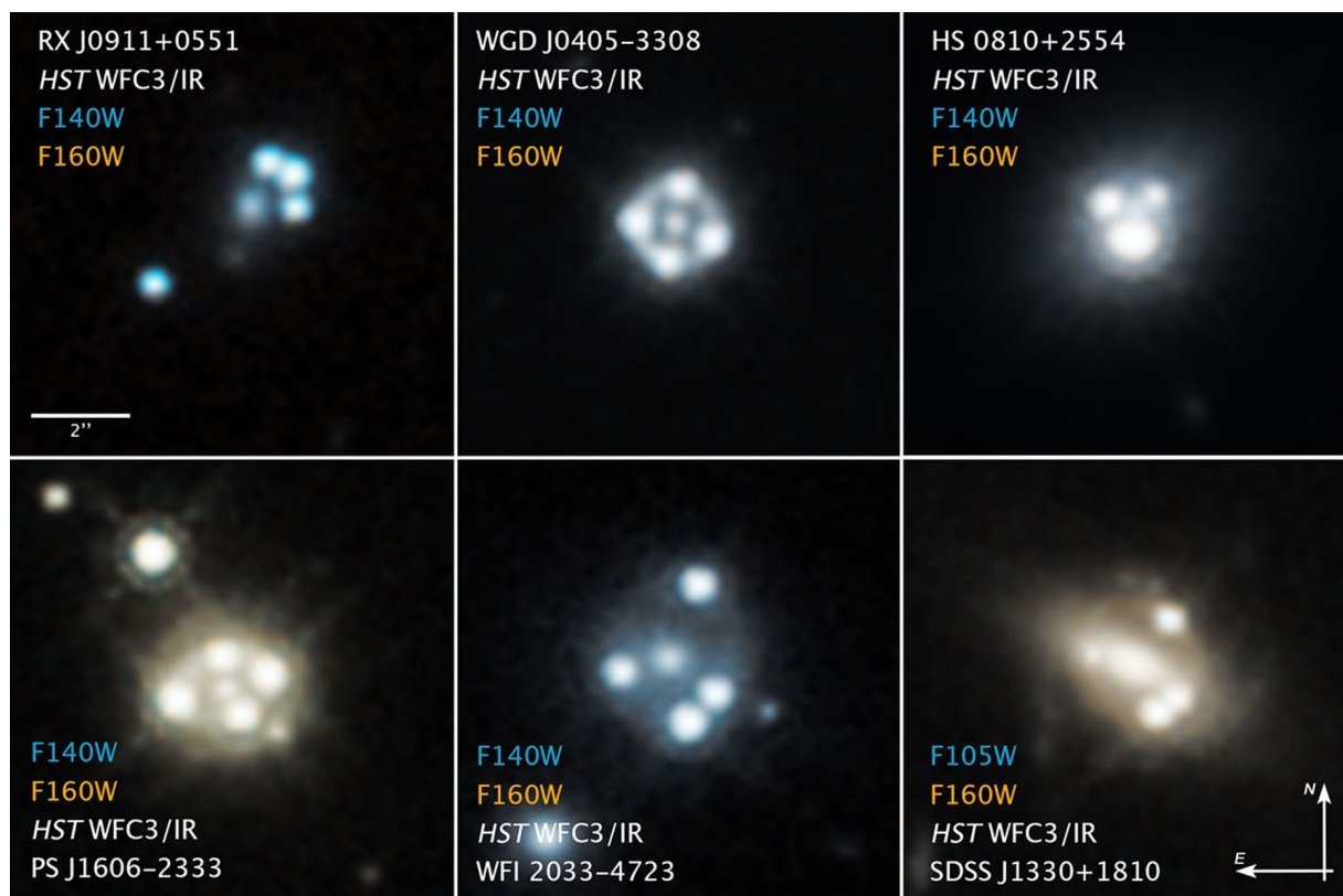
Figure 20. Compass Image of Gravitationally Lensed Quasars
